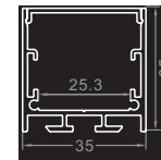
Installation Diagram
