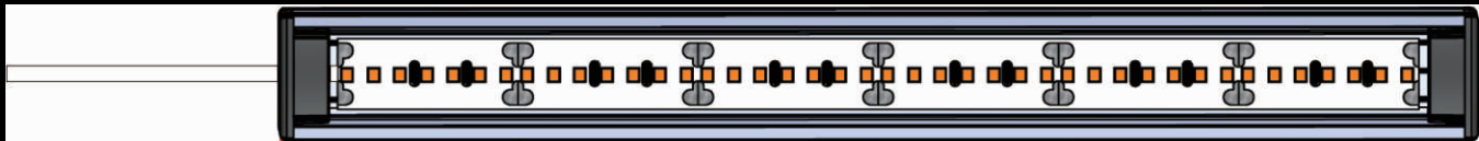
End Cap Length Extra Profile Length LED Strip Length Extra Profile Length End Cap Length
