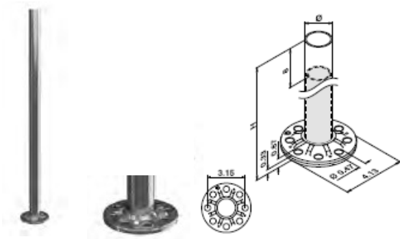
1.5" DIAMETER DOUBLE WALL THICKNESS 0.156" HEIGHT 38"
