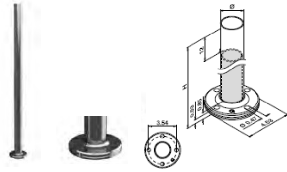
1.9" DIAMETER DOUBLE WALL THICKNESS 0.156" HEIGHT 42"
