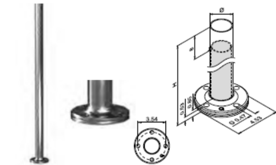
1.9" DIAMETER DOUBLE WALL THICKNESS 0.156" HEIGHT 38"
