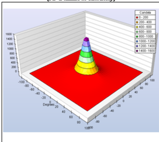
(3D Luminous Intensity)
