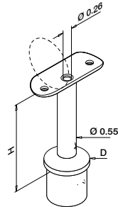
SR 0702 - D = Ø 1-1/2" x 0.078 (38.1 x 2.0 mm)
