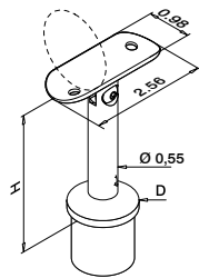
SR 0705 - D = Ø 1-1/2 x 0.078 (38.1 x 2.0 mm)
